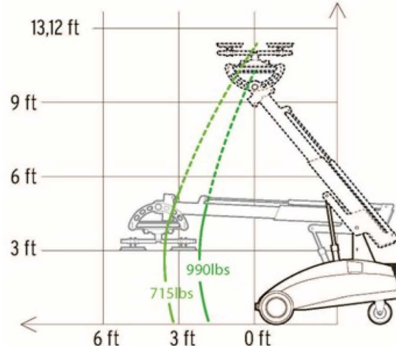
PICKUP AND PLACE DIAGRAM
